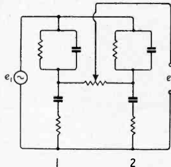
Fig. 5 Output taken across series-connected elements.
