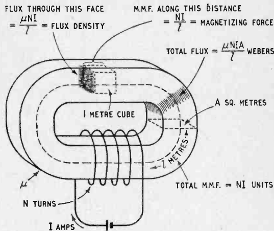
Showing the simple relationships between magnetic units in the rationalized m.k.s. system. The usual mixed "practical" and c.g.s. system necessitates various constant factors composed of 10 and 4\pi .
