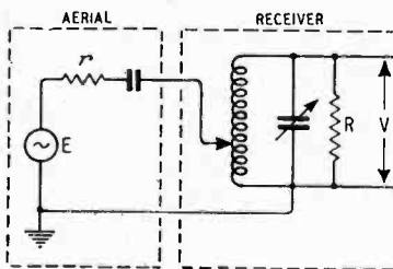
Fig. 3. R is the value of the dynamic resistance of the tuned circuit (with aerial disconnected) together with the valve input resistance and any other losses, for purposes of calculating maximum signal voltage V .
