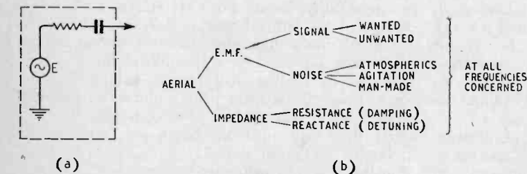
Fig. 1. The equivalent circuit of an aerial (a), and its properties and products analyzed (b)
