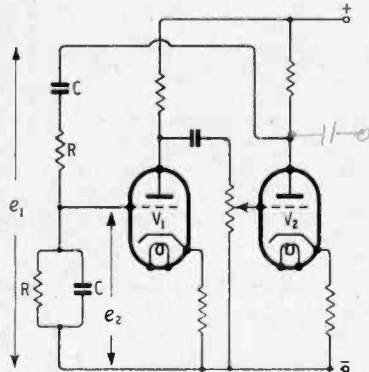
Fig. 1 Basic Wien bridge R-C oscillator.
