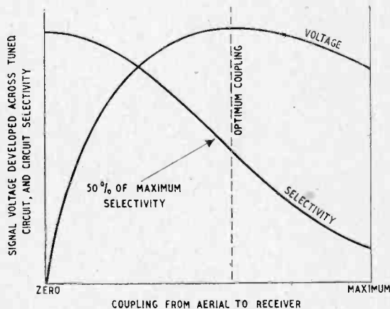
Fig. 4. Typical effect on signal voltage across the pre-selector tuning circuit, and on its selectivity, of varying the aerial coupling.
