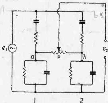
Fig. 2 Combination of two dissimilar frequency discriminating networks.
